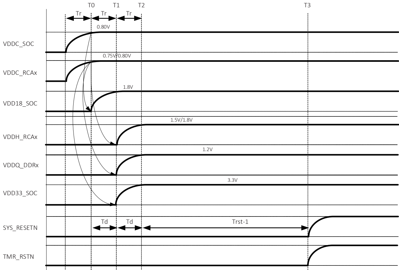
Figure 4: Power-on Voltage Sequencing – SoC Domain
